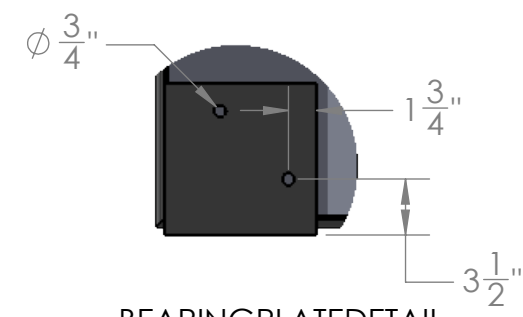
BEARING PLATE DETAIL SCALE 1 : 12
