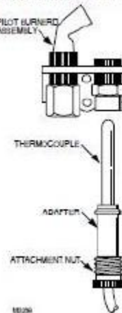
Fig. 5—Installing Q390 Thermocouple.
