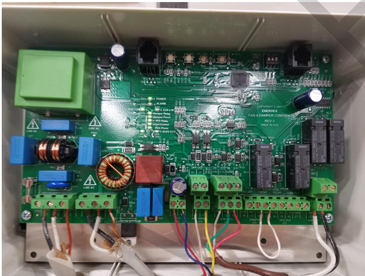
Picture 8 – Custom Gas L-Shaped Fireplace Draft Control Component
